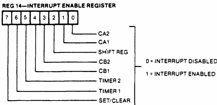
Figure 37. Interrupt Flag Register (IFR)
